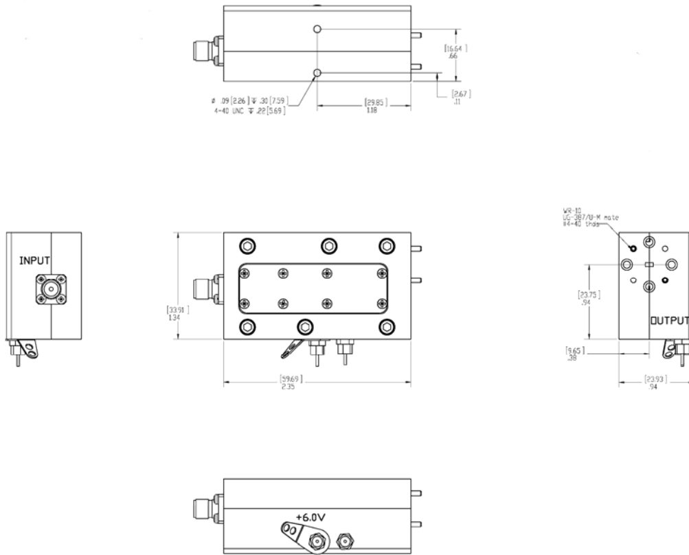
W-Band X6 Active Multiplier
